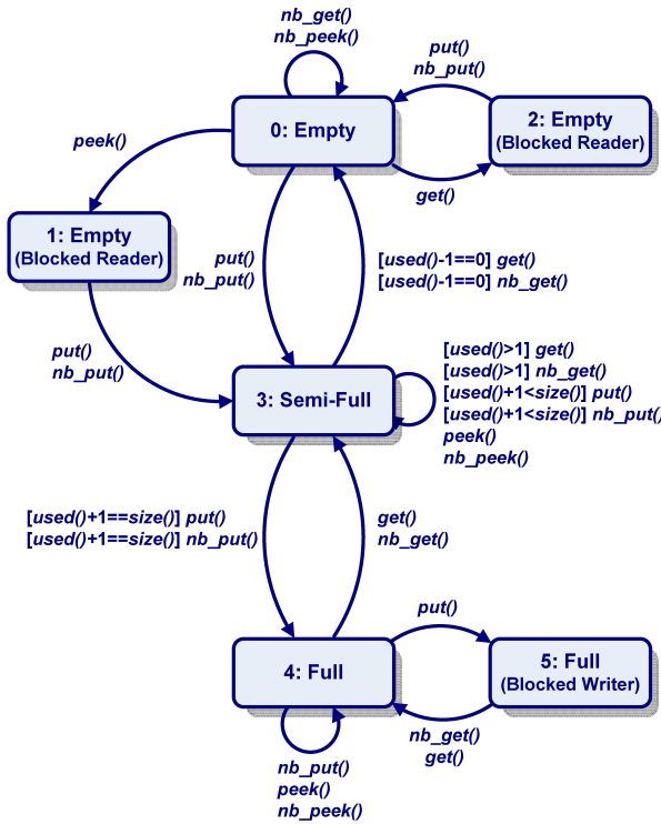
Figure 5 tlm_fifo UML State Chart
